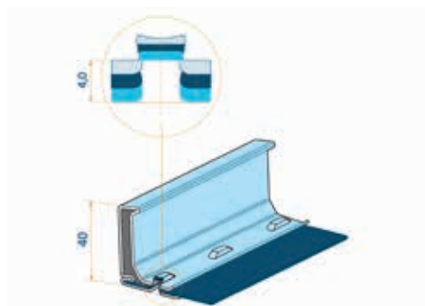
Luftkanal-Schnitt 3-lagig / 3-layer airduct cross-section
